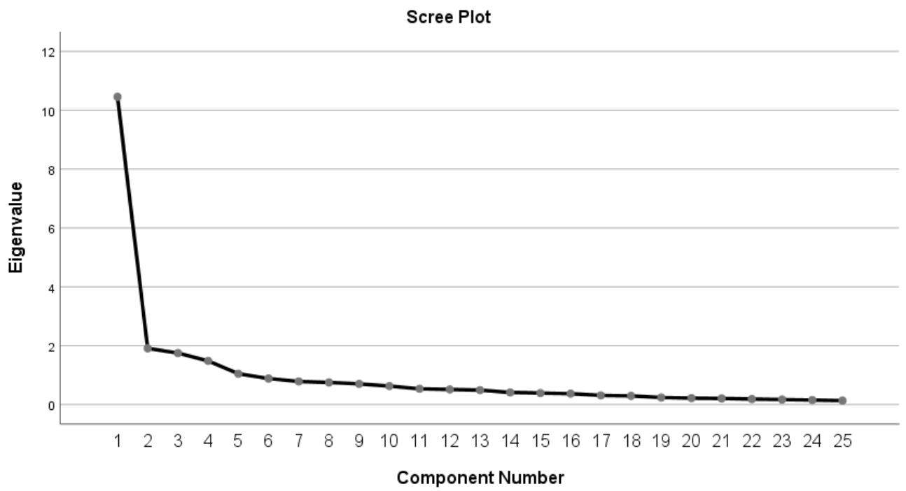
Fig. S3. Scree plot test.
